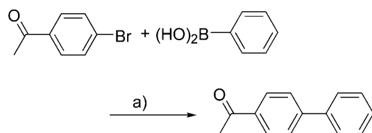
Scheme 3. Suzuki coupling reaction performed with the supramolecular palladium complex 4 . a) 0.1, 0.5 and 1 mol % catalyst (see Table 1), Na 2 CO 3 , DMF, 80 °C, 20 h.
